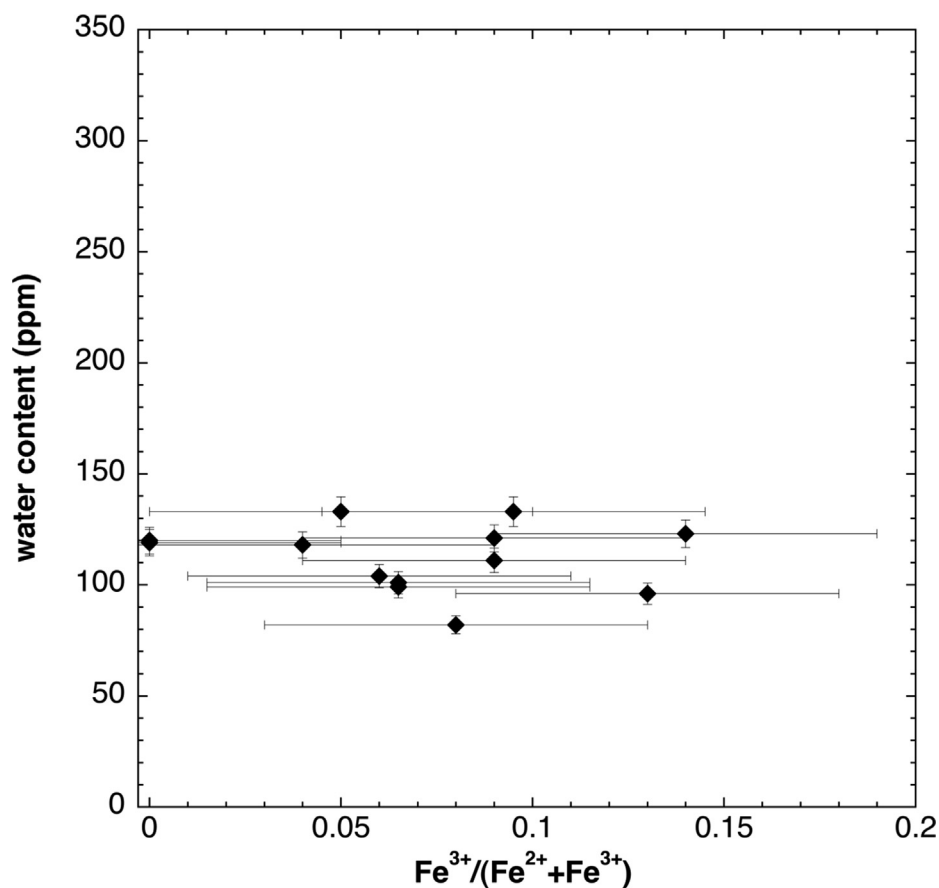
Fig. 13. Water content of the studied Belize glasses vs. XAS-derived \text{Fe}^{3+}/(\text{Fe}^{2+}+\text{Fe}^{3+}) ratio. Both the water content (ranging from 80 to 132 ppm) and the \text{Fe}^{3+}/(\text{Fe}^{2+}+\text{Fe}^{3+}) ratio are consistent with literature data on tektites.
