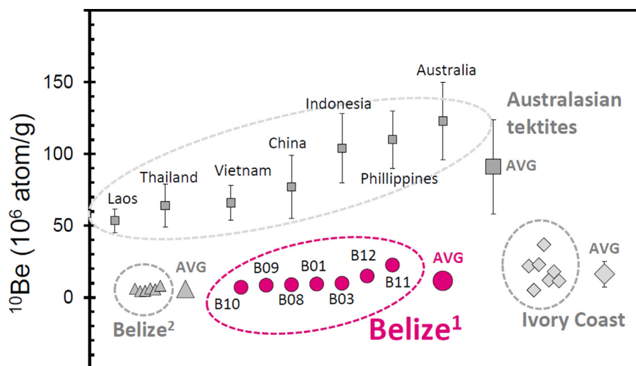
Fig. 14. ^{10}\text{Be} concentrations of Belize tektites and other tektites. All concentrations are re-normalized to a ^{10}\text{Be} half-life of 1.36 Ma (Nishiizumi et al., 2007). Belize 1 (this work), Belize 2 (Rochette et al., 2021), Australasian tektites (Ma et al., 2004), Ivory Coast (Serefidin et al., 2007). The x-axis has no general significance, except that for Australasian tektites the data are plotted with increasing distance from the central Indochina region.
