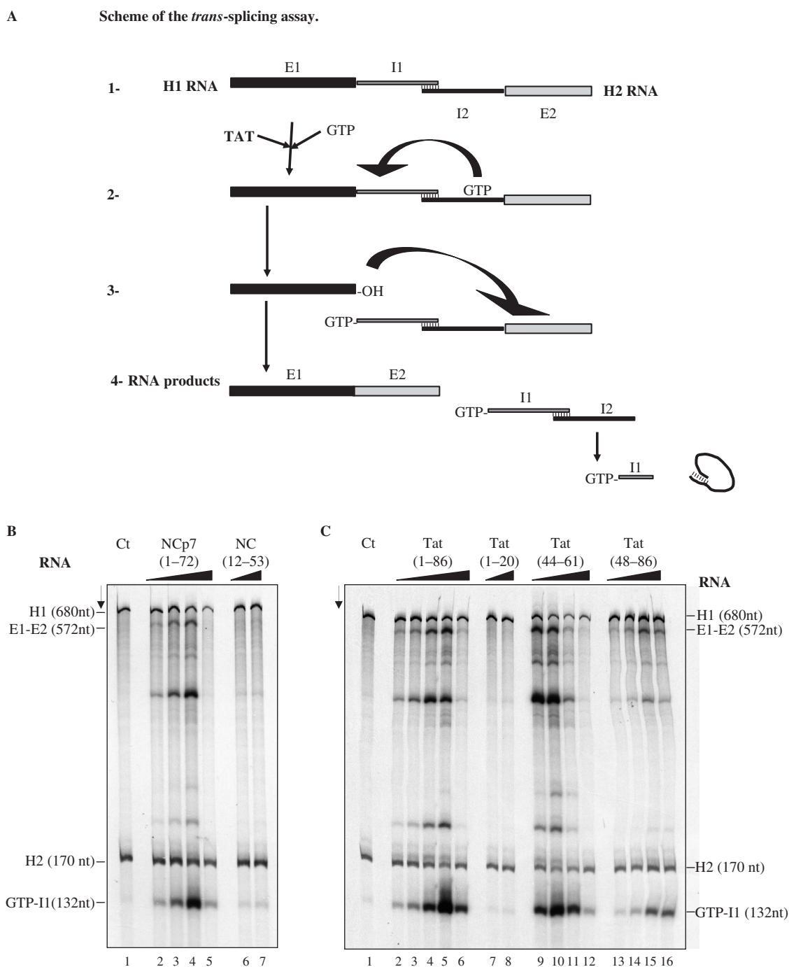
Figure 6. Enhancement of trans -splicing by HIV-1 Tat. (A) Schematic representation of the trans -splicing assay: The two RNA constructs H1 (encoding exon 1 and the 5' part of the intron) and H2 (encoding the 3' part of the intron and exon 2) have to fold into a splicing competent structure (1). The splicing reaction was started by addition of the ^{32}\text{P} -labeled GTP. The nucleic acid chaperone was eventually added at step 2. The final RNA products are represented in (4). The splicing rates are based on the levels of GTP-I1 (see B). (B and C) Assays where the H1 and H2 RNAs were incubated with or without a nucleic acid chaperone. At the end of the reaction RNAs were phenol treated to remove the protein and analysed by PAGE in denaturing conditions (see Materials and methods section). The RNA substrates (H1, H2), the ligated exons (E1-E2) and the product (guanosine-5'-intron G-I1) are indicated. Panel B. Lane 1: splicing reaction at 37^\circ\text{C} with RNA alone at a concentration of 4 \times 10^{-8}\text{ M} . Lanes 2–5: HIV-1 NCp7 at concentrations of 2.5, 5, 10 and 20 \times 10^{-7}\text{ M} , corresponding to protein to nt ratios of 1:128, 1:64, 1:32 and 1:16. Lanes 6 and 7: NC(12–53) at concentrations of 1 and 2 \times 10^{-6}\text{ M} , corresponding to peptide to nt ratios of 1:32 and 1:16. Panel C. Lane 1: splicing reaction at 37^\circ\text{C} with RNA alone at a concentration of 4 \times 10^{-8}\text{ M} . Lanes 2–6: Tat(1–86) at concentrations of 1.25, 2.5, 5, 10 and 20 \times 10^{-7}\text{ M} , corresponding to protein to nt molar ratios of 1:256, 1:128, 1:64, 1:32 and 1:16. Lanes 7 and 8: Tat(1–20) at concentrations of 1 and 2 \times 10^{-6}\text{ M} . Lanes 9–12: Tat(44–61) at concentrations of 2, 4, 8 and 16 \times 10^{-7}\text{ M} , corresponding to peptide to nt molar ratios of 1:170, 1:85, 1:42.5 and 1:21.2. Lanes 13–16: Tat(48–86) at concentrations of 2, 4, 8 and 16 \times 10^{-7}\text{ M} , corresponding to molar ratios of 1:170, 1:85, 1:42.5 and 1:21.2. Note that HIV-1 NCp7 and Tat strongly activated trans -splicing at protein to nt molar ratios of 1:32 (compare lanes 1 and 4 in B, and lanes 1 and 5 in C). Tat peptide (44–61) was also very active (lane 10 in C). Peptides NC(12–53) and Tat(1–20) were very poorly active.
