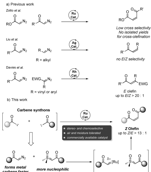
Scheme 1. Previously reported cross-olefinations and this work.
