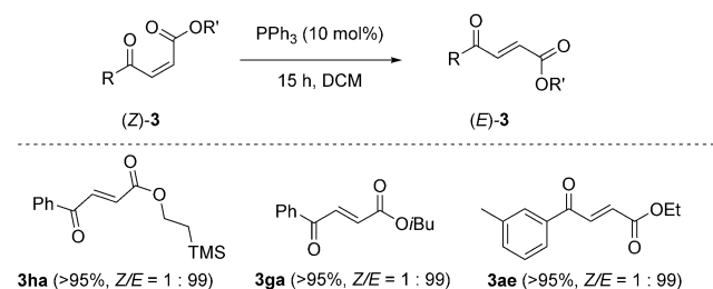
Scheme 6. Isomerization to E olefins.
